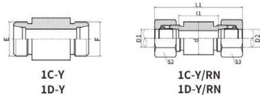
圆柱过板接头 CYLINDER STRAIGHT BULKHEAD
