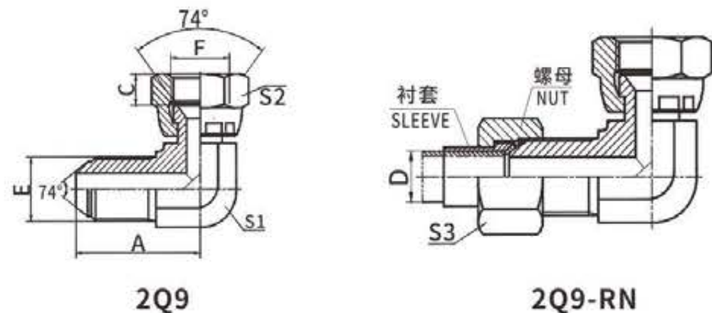
公制外螺纹74°外锥/公制丙螺纹74°内锥 METRIC MALE 74° CONE / METRIC FEMALE 74° SEAT
